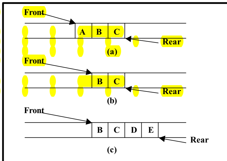
Fig 8.18: A queue
